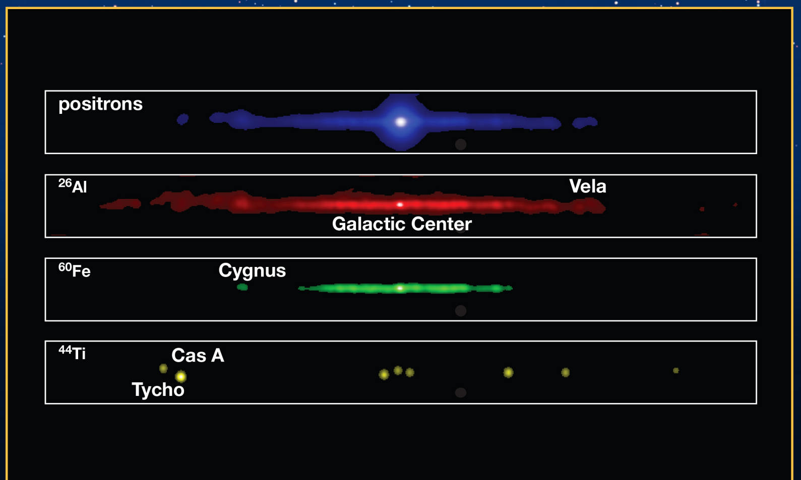
Simulated COSI images of our Galaxy showing gamma-rays from antimatter annihilation (blue, top) and Aluminum (red, middle-top), Iron (green, middle-bottom), and Titanium (yellow, bottom). These products are created during the evolution of massive stars.
