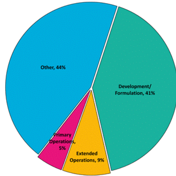
Earth Science
