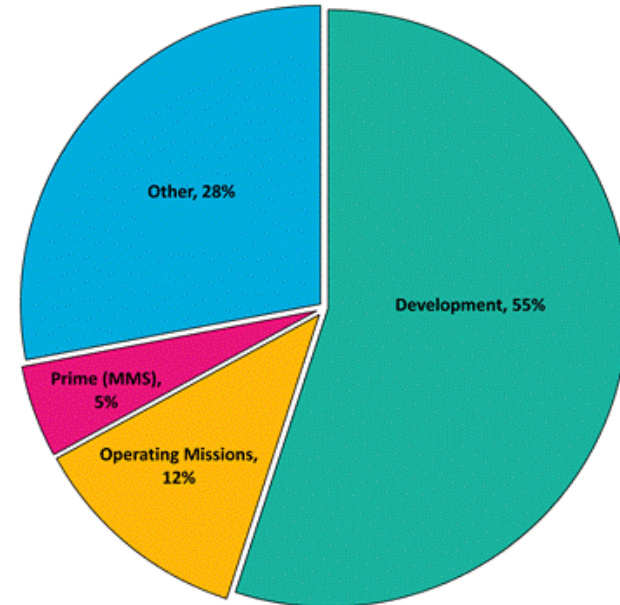
Heliophysics
