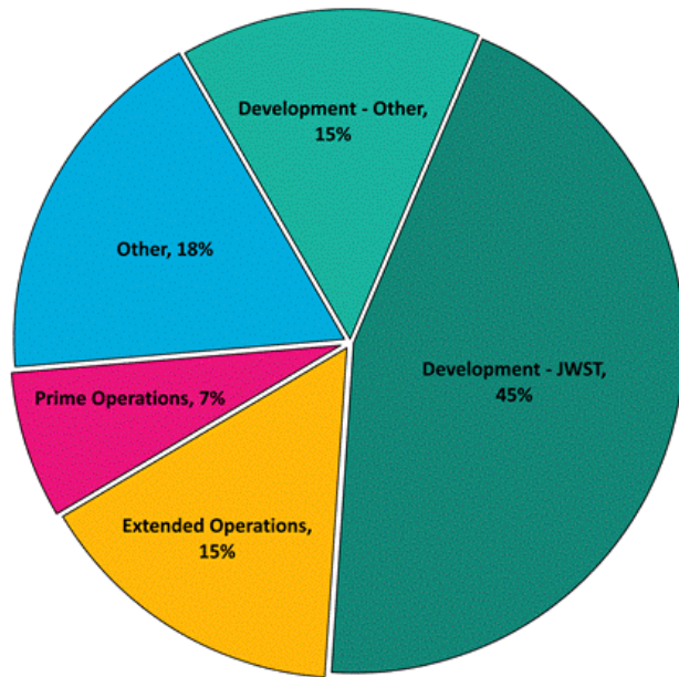
Astrophysics
