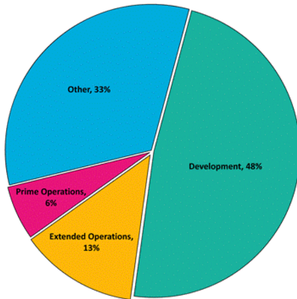
Planetary
