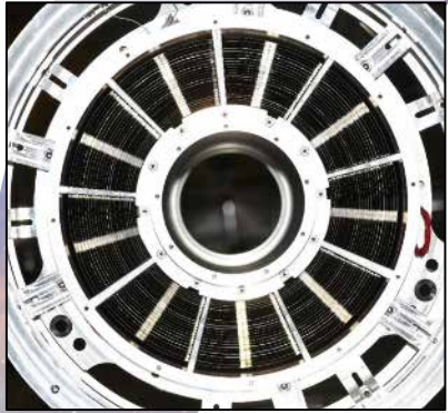
MMA 24 X-ray shells edge-on front view
