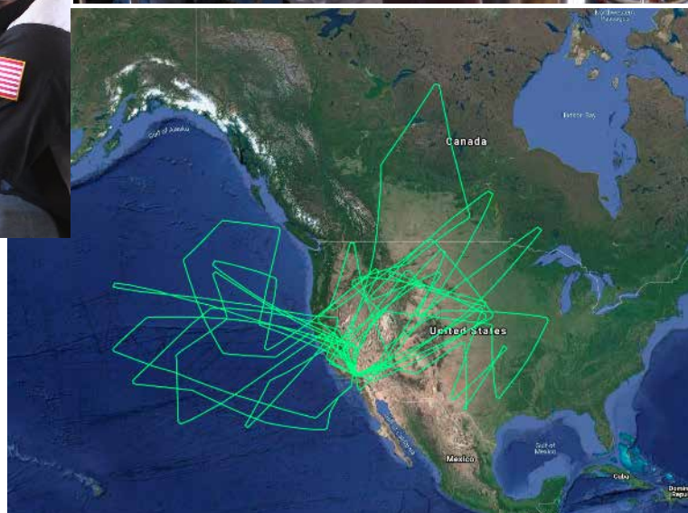
Flight paths of the 15 science flights
