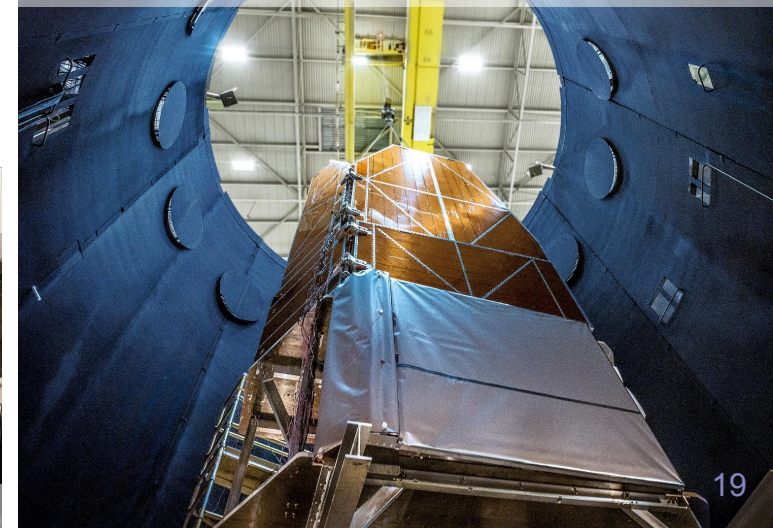
Solar Array / Sun Shield Engineering Test in Thermal/Vacuum Chamber
