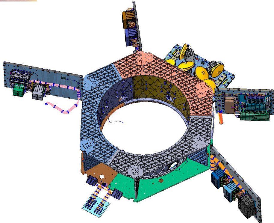
Deployable Aperture Cover Engineering Test
