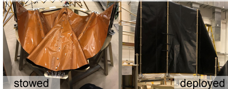
Deployable Aperture Cover Engineering Test
