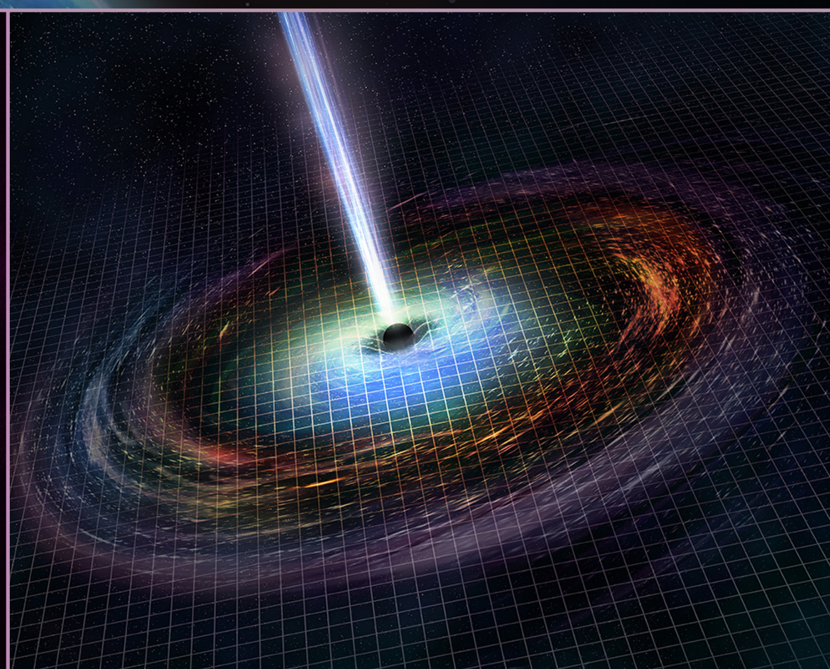
Artist's illustration of a black hole emitting a jet of high-energy particles, surrounded with a disc of infalling matter
