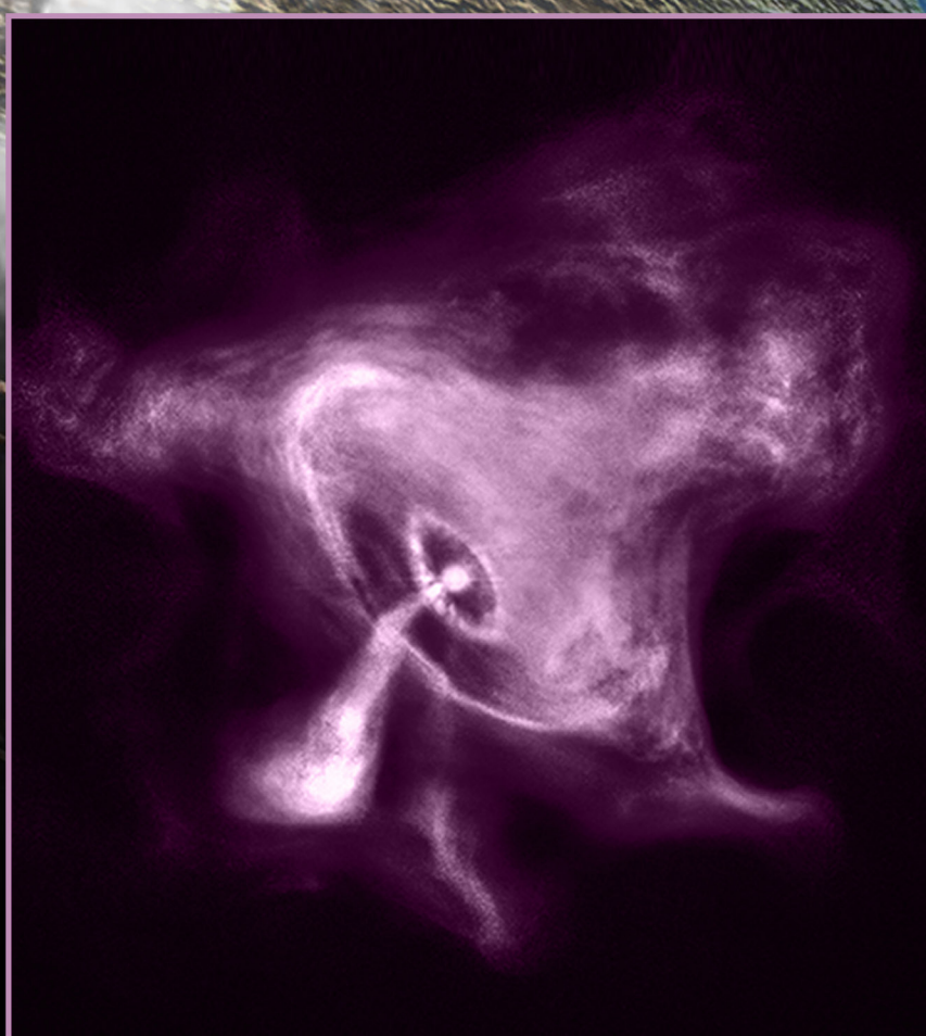
X-ray view of the Crab Nebula, powered by highly magnetized neutron star called a pulsar
