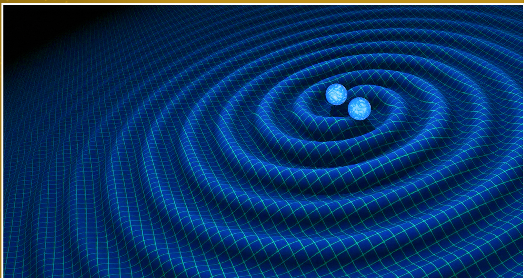
Artist's impression of gravitational waves generated by binary neutron stars
