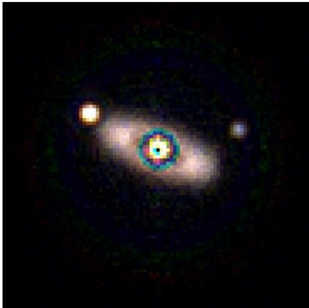
Altair 12 hrs each in V, R, I bands. Jupiter & Saturn analogs detected, 1 zodi dust ring from 2-4 AU
