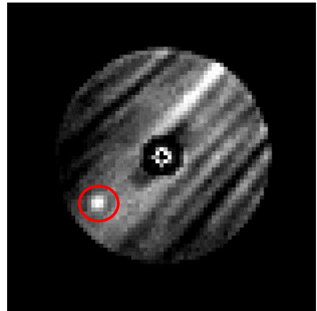
5 day V band exposure of an Earth analog in the HZ of \alpha Cen A (occulted at center). Scattered light from \alpha Cen B is the primary noise source; shown is a 3% residual after calibration.
