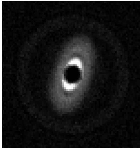
12 hr V band exposure of HIP 85790, a V= 5.6 star at 80 pc with WISE infrared excess. A 50 zodi debris disk extended to 80 AU radius is assumed.
