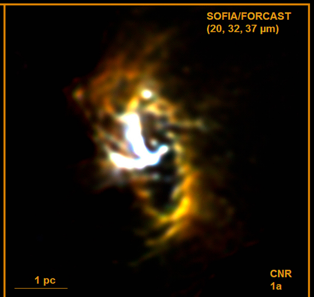
Milky Way Galaxy Black Hole Circumnuclear Ring – 2013
