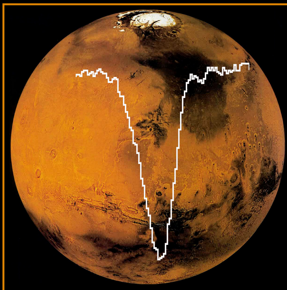
First detection of atomic oxygen in Mars atmosphere in 40 years – 2015
