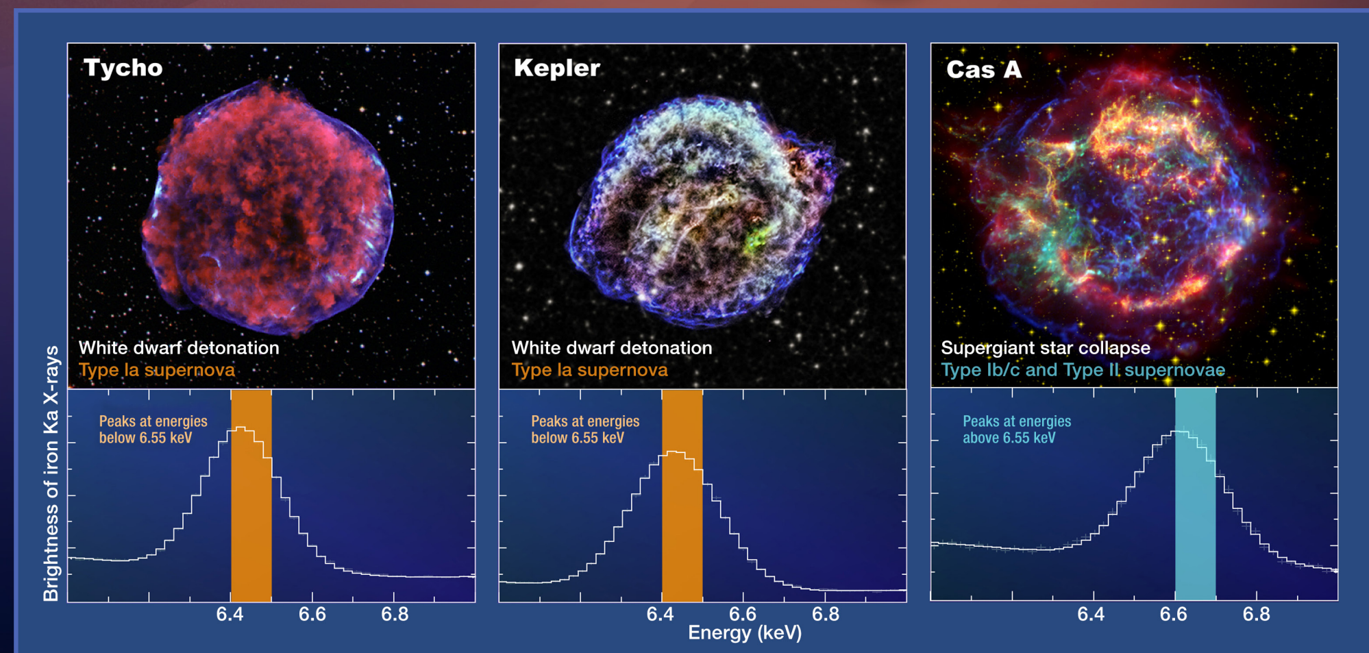
X-ray energies in supernova remnants
