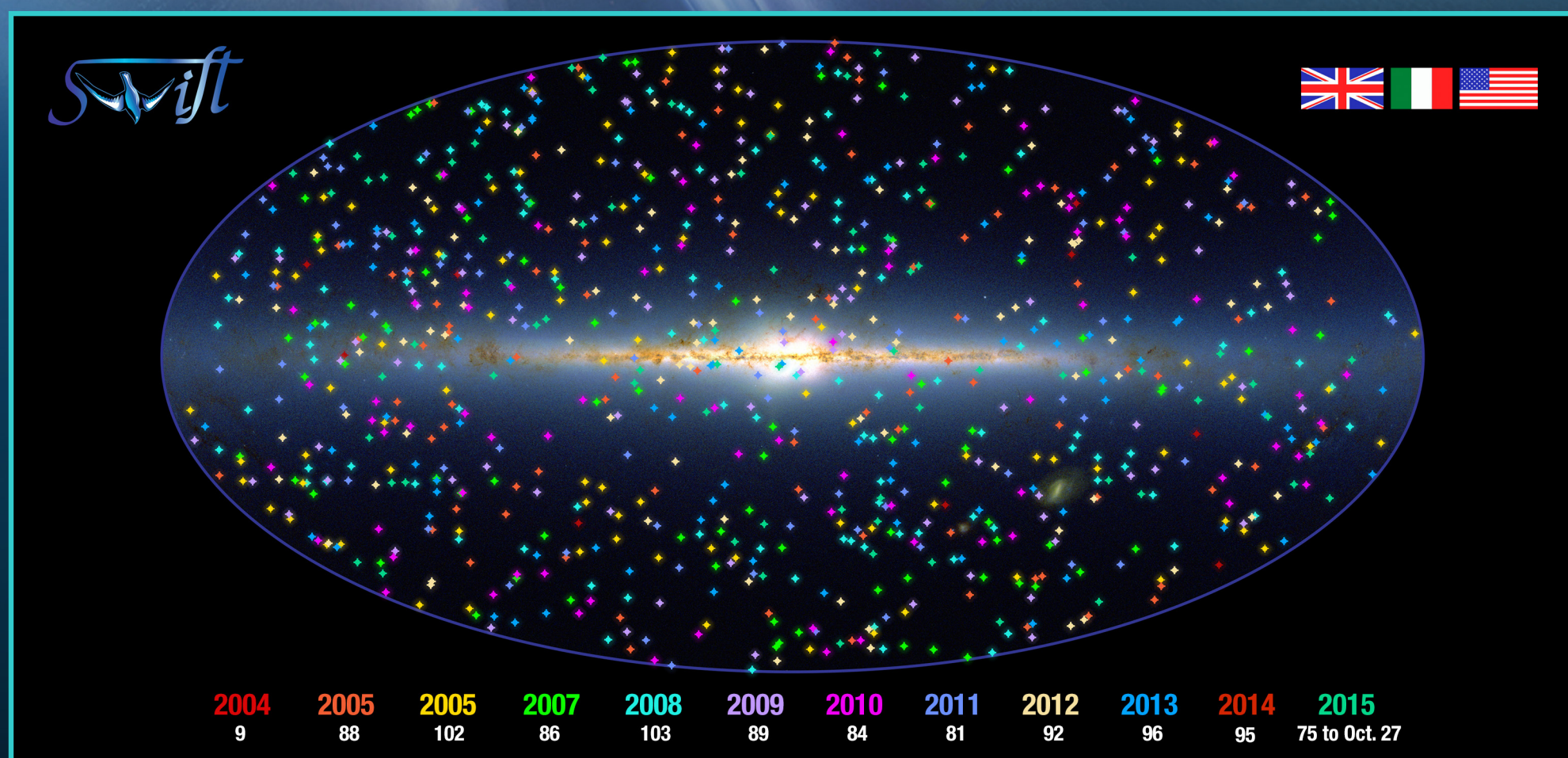
Map of the sky showing the first 1,000 gamma-ray bursts detected by Swift – November 6, 2015
