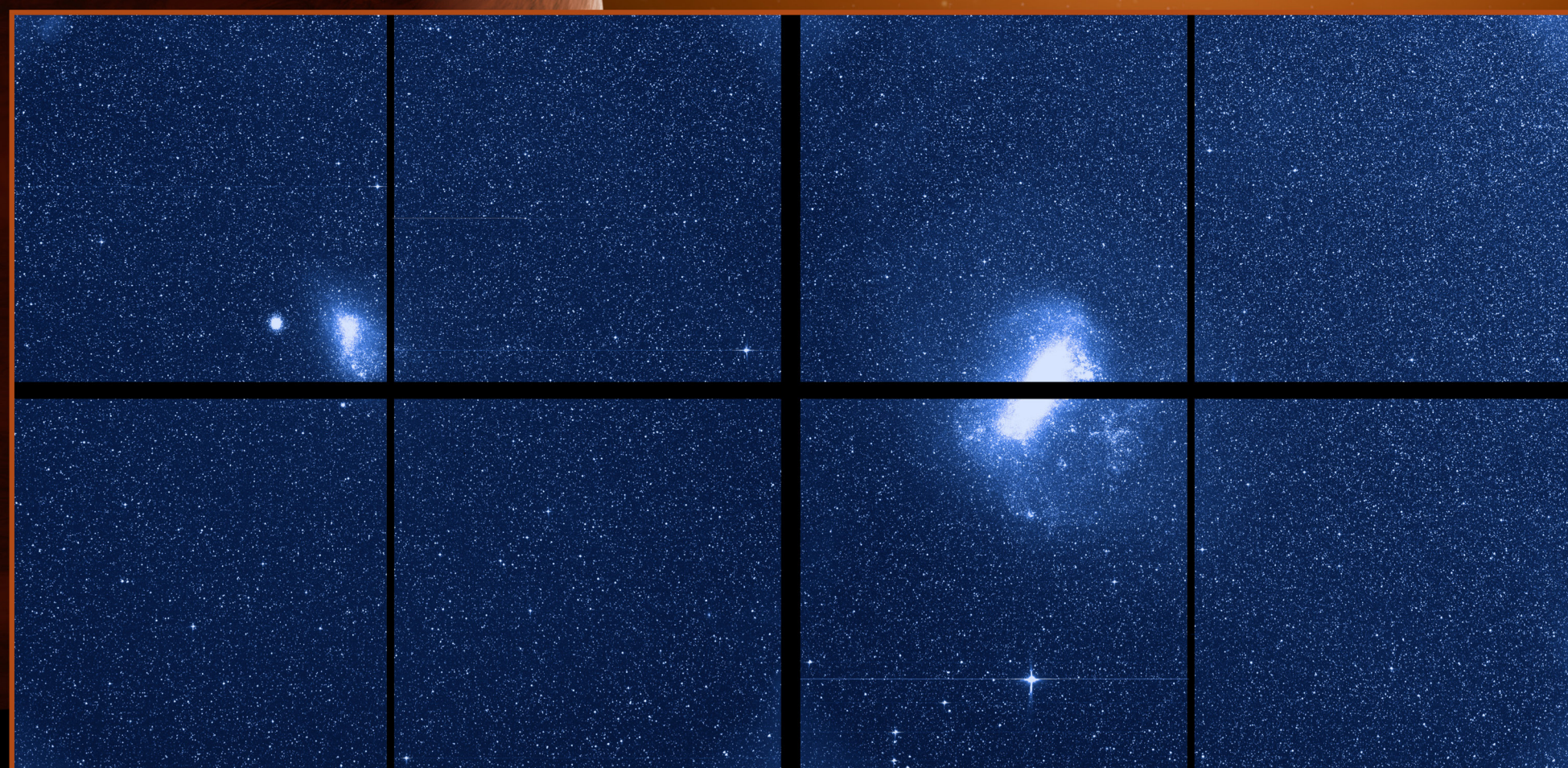
TESS's wide field-of-view cameras are surveying our galactic neighborhood for transiting exoplanets.
