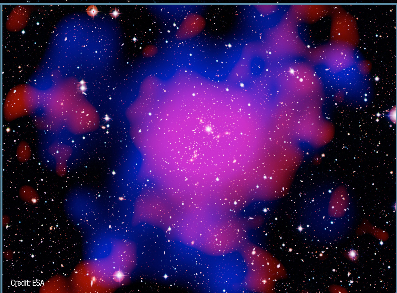
Galaxy Cluster Abell 2744 – December 2, 2015
