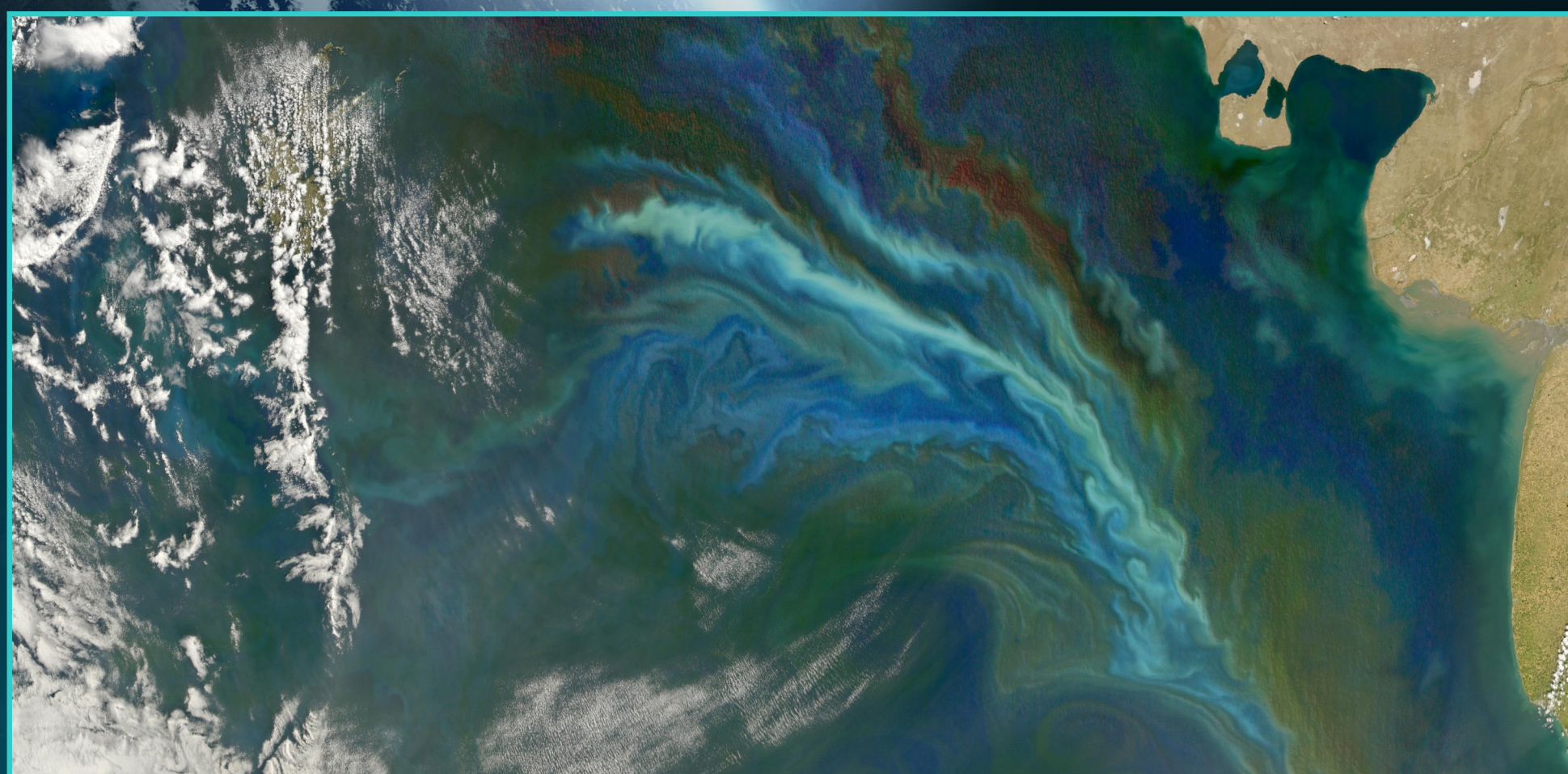
Phytoplankton blooming off the Atlantic Coast – December 21, 2010
