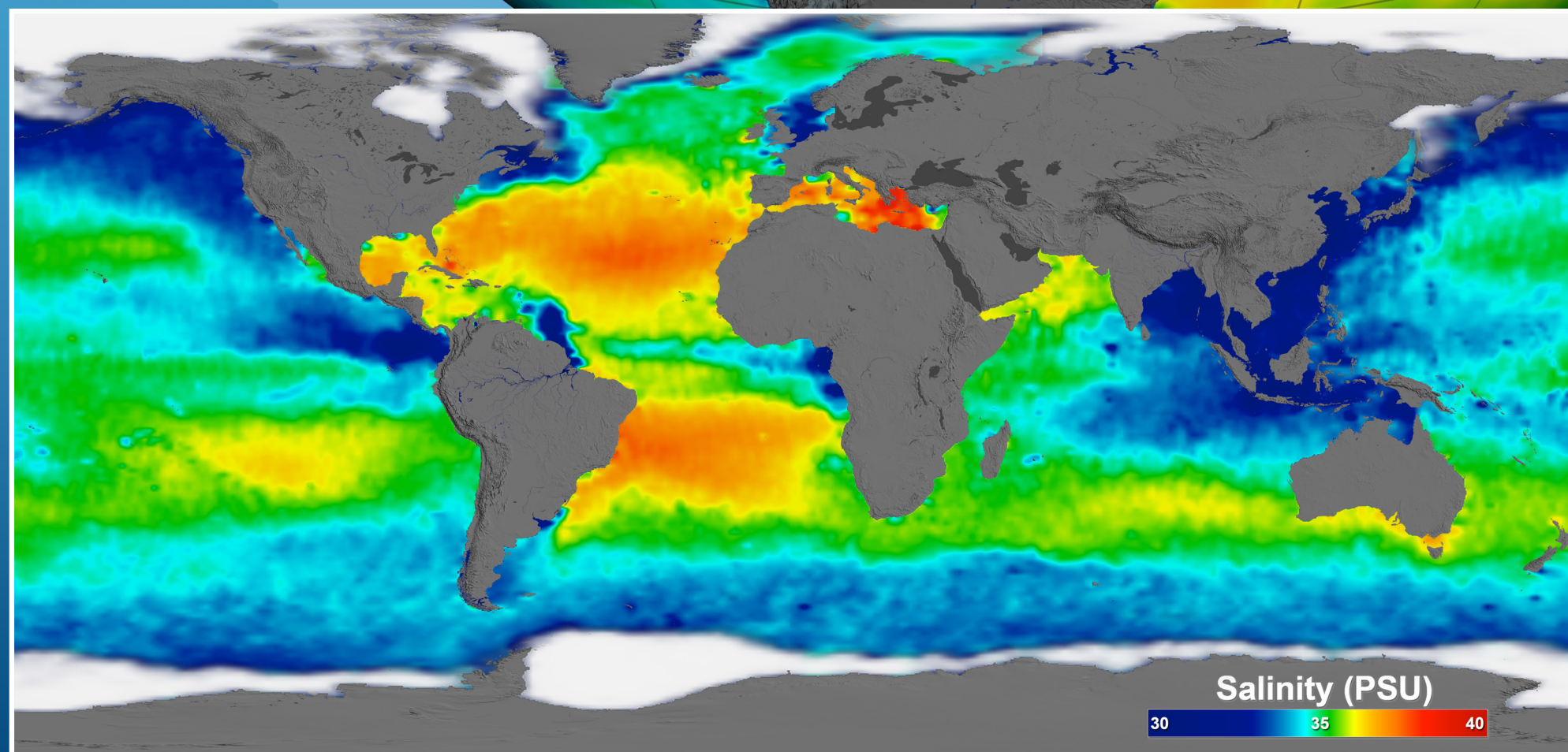
Flat map projection of Aquarius sea surface salinity data – between September 2011 and September 2014
