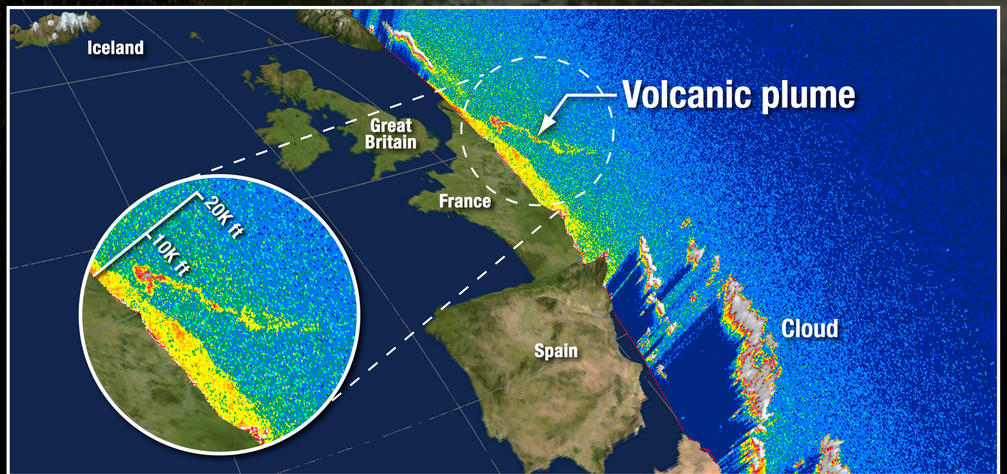
CALIPSO watches Eyjafjallajökull's plume drift over northern Europe – April 17, 2010
