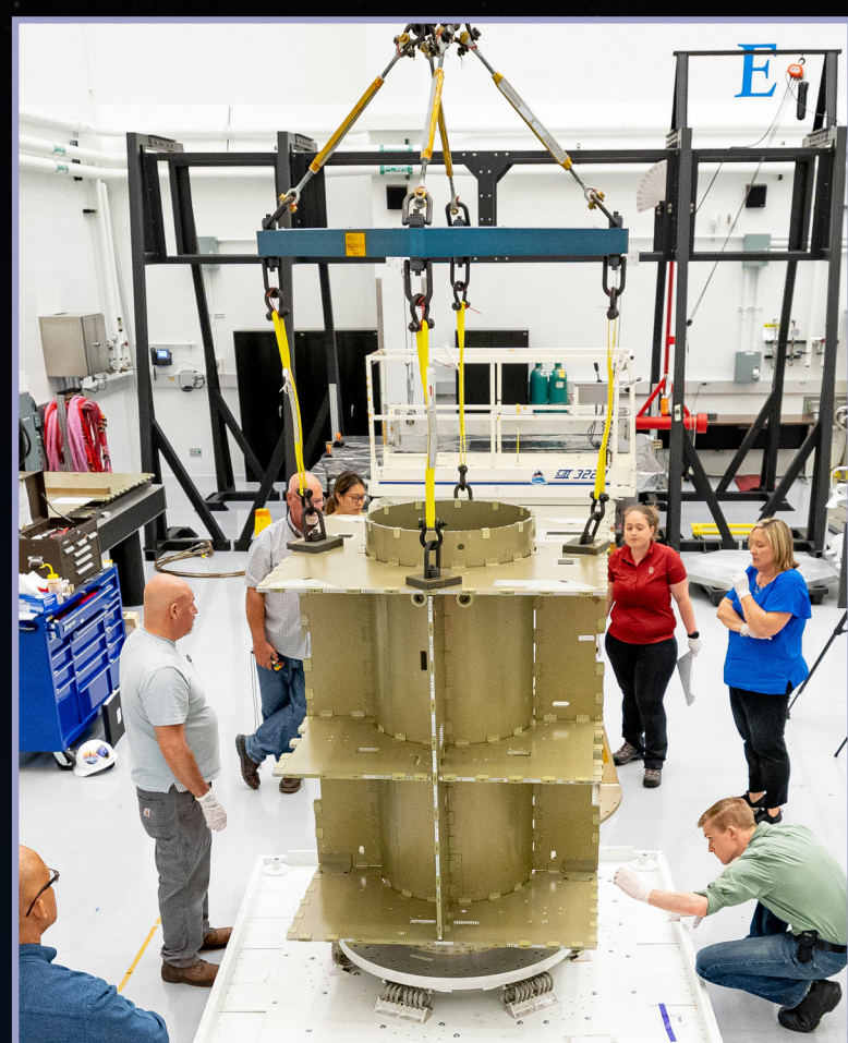
Spacecraft body in APL high bay – July 2019
