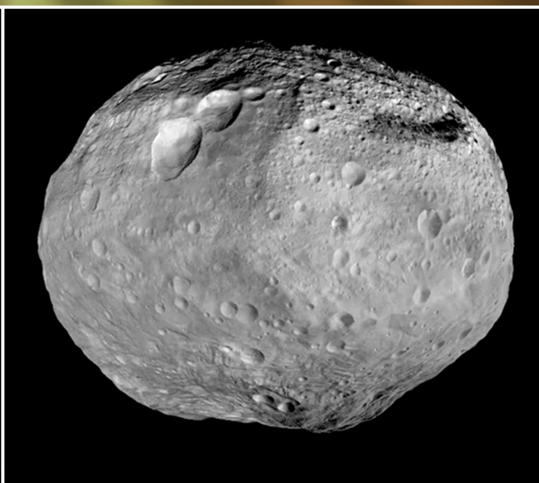
Protoplanet Vesta – July 2011-September 2012
