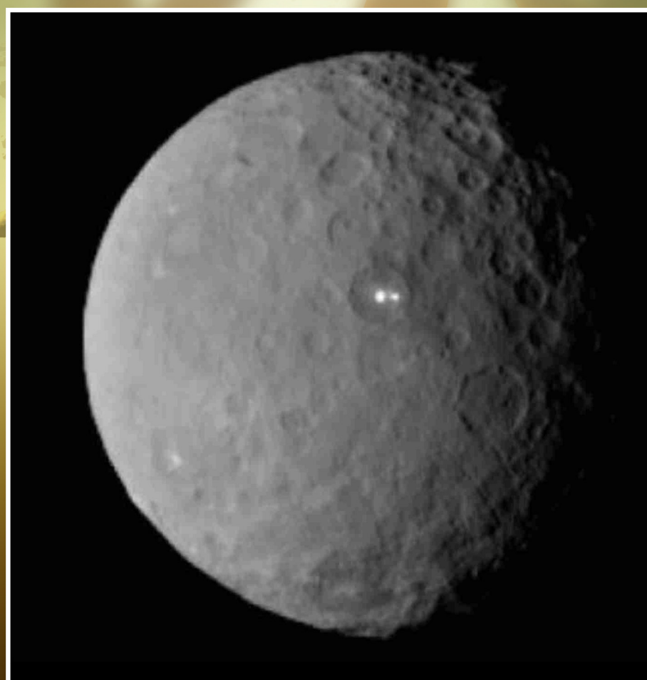
Dwarf Planet Ceres – February 19, 2015
