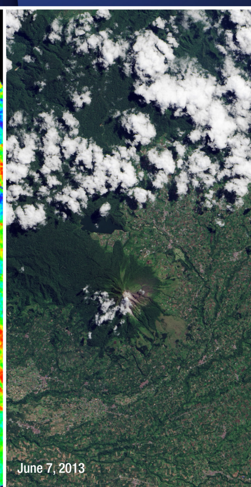
Advanced Land Imager (ALI) views changed landscape around Indonesia's Sinabung Volcano
