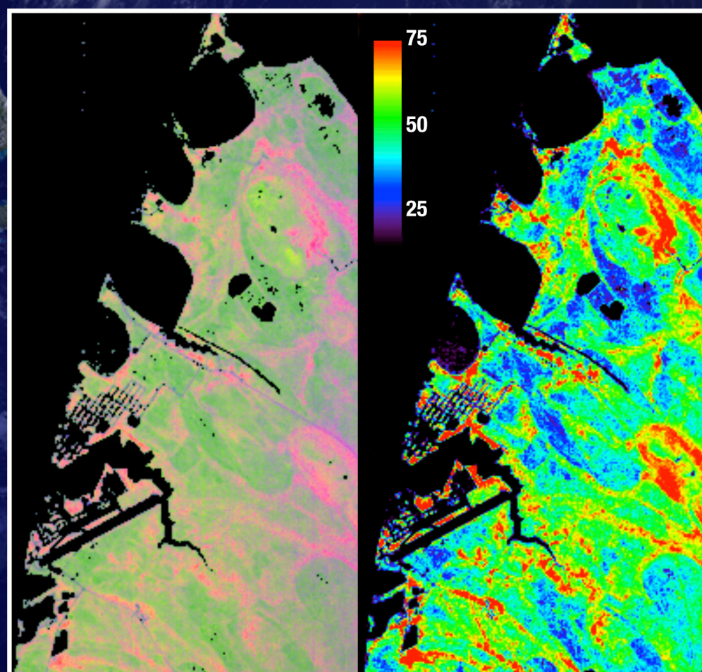
Hyperion maps of plant functional types (left) & photosynthetic efficiency (right) of tundra near Barrow, Alaska – July 20, 2009
