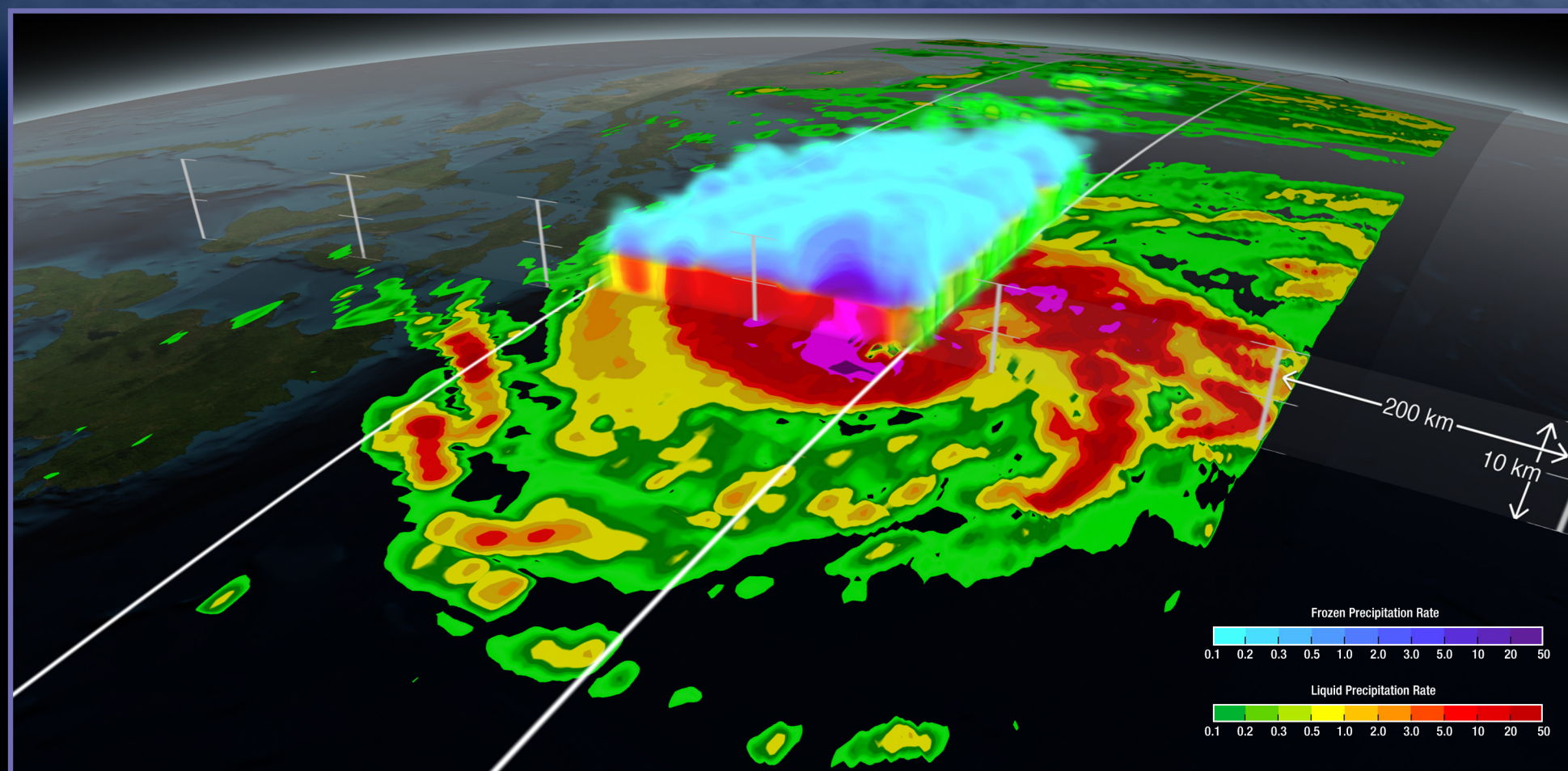
Super Typhoon Hagupit from the GPM Microwave Imager (surface map) and Dual-frequency Precipitation Radar (3-D data) aboard the GPM Core Observatory – December 5, 2014
