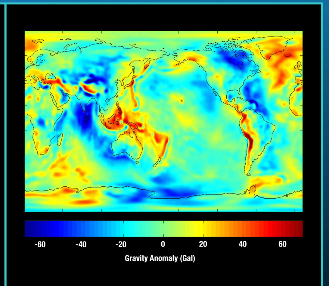
Earth's Gravity Field Map – 2003
