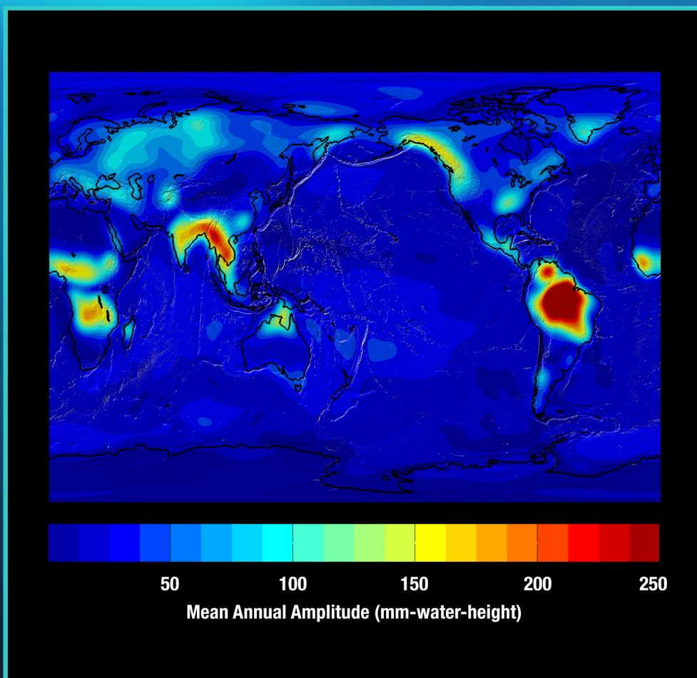
Mean Annual Amplitude – 2002 to 2016
