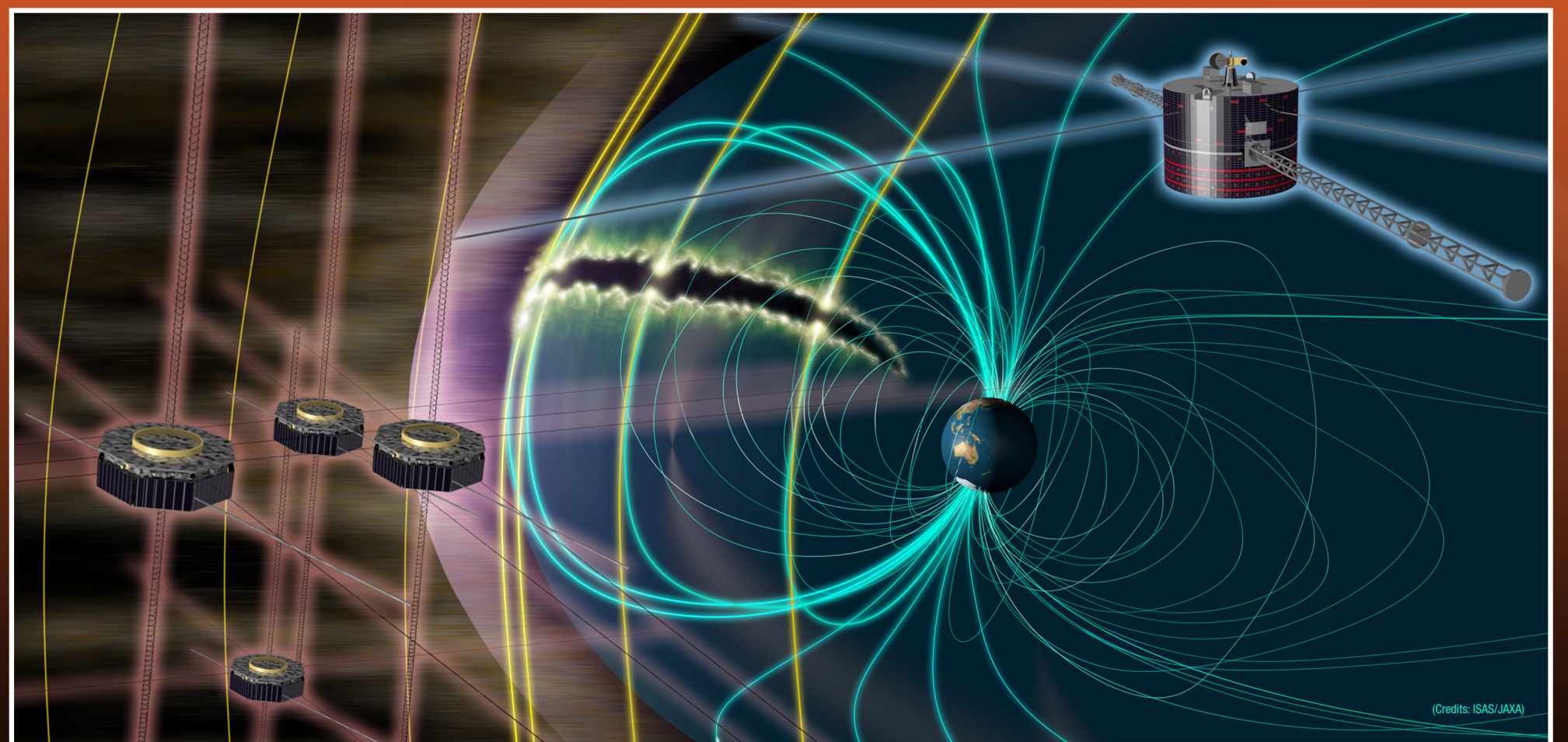
Artist concept of the Geotail and MMS missions studying how the Earth's magnetosphere takes in solar wind energy.
