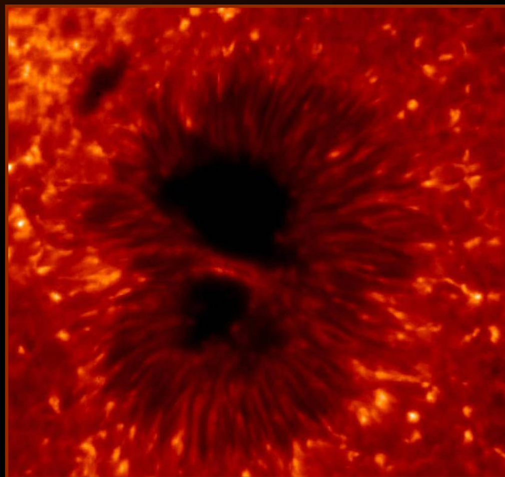
Sunspot – September 23, 2014
