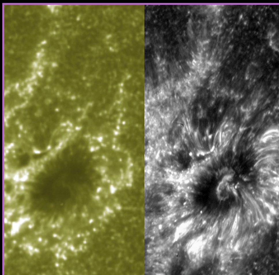
SDO ultra violet image (right) compared to IRIS seen in the light of three times ionized Silicon (left) – July 25, 2013
