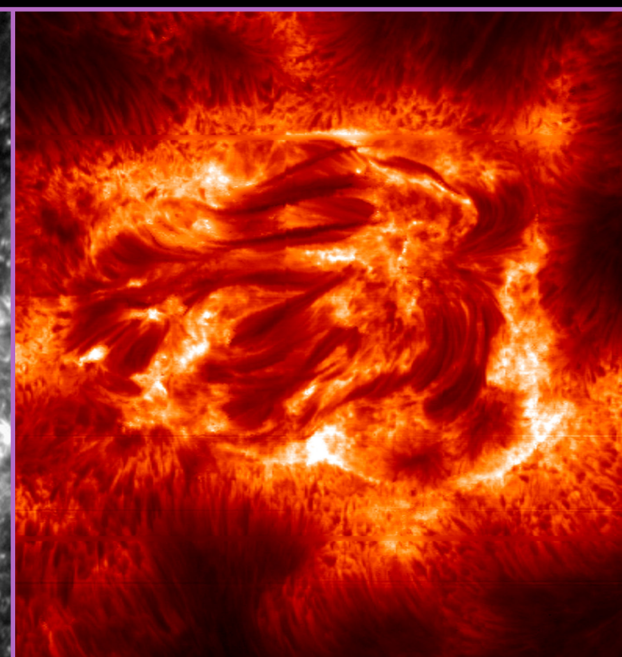
An active region on the Sun from IRIS in the light of singly-ionized Magnesium – December 6, 2013
