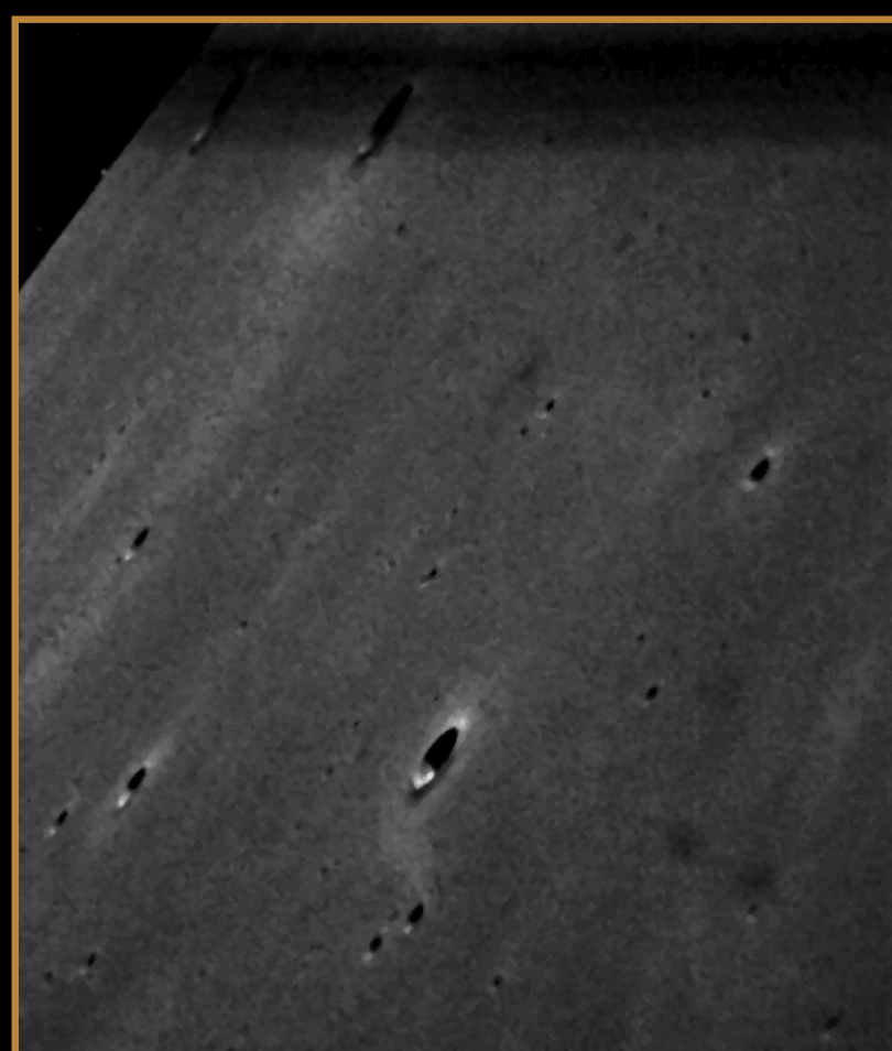
Craters Lichtenberg A & Schiaparelli E – February 8, 2014
