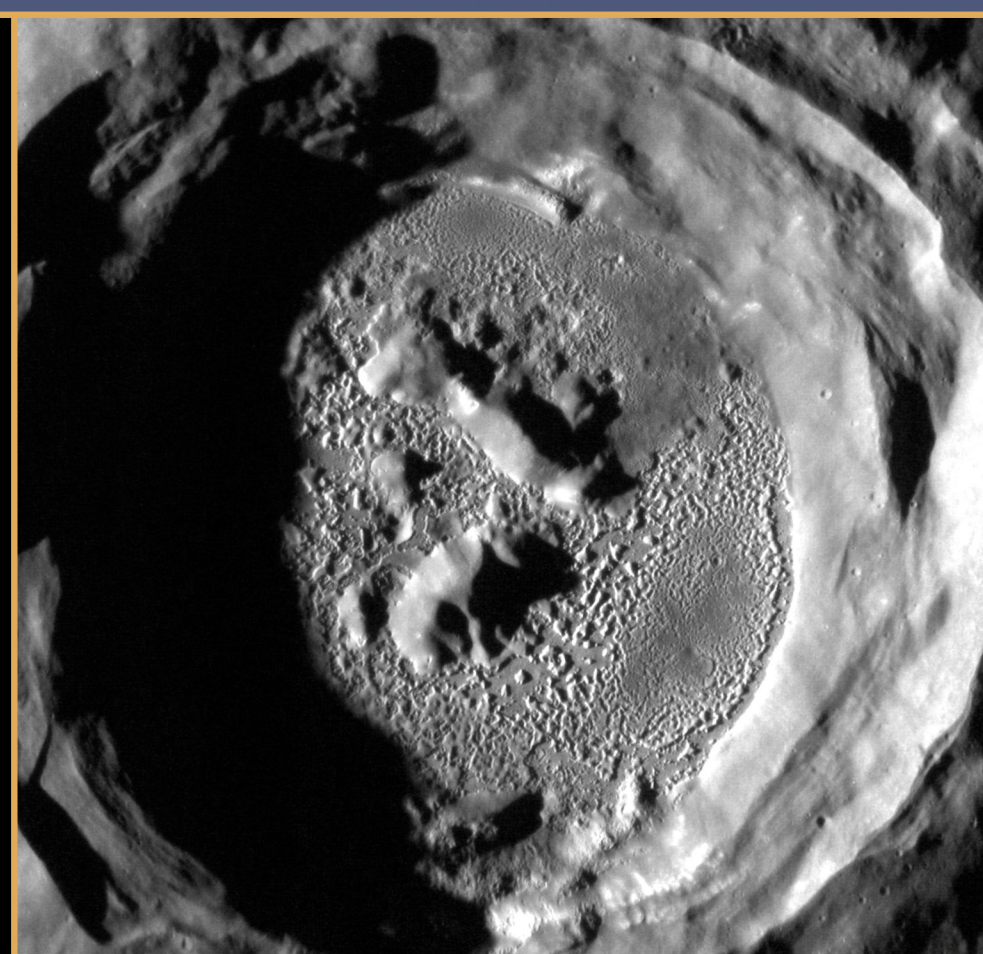
Kertesz Crater – January 25, 2013
