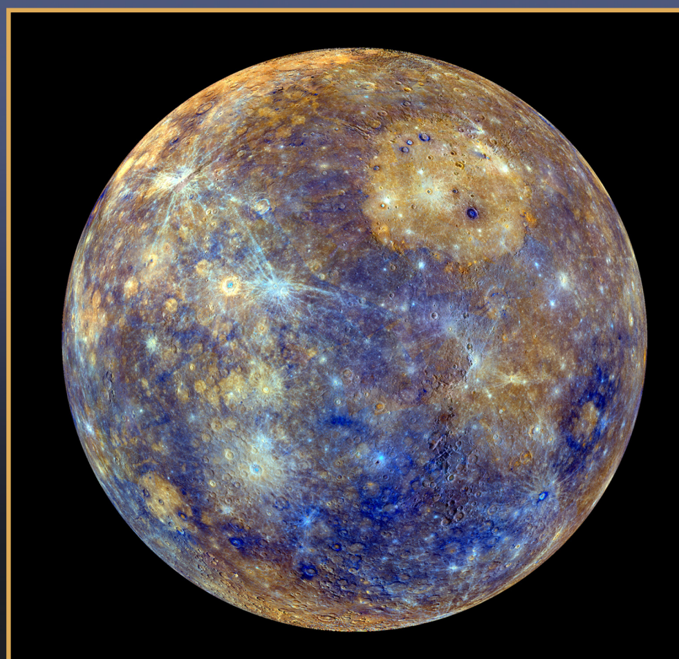
Mercury in Enhanced Color – February 18, 2013
