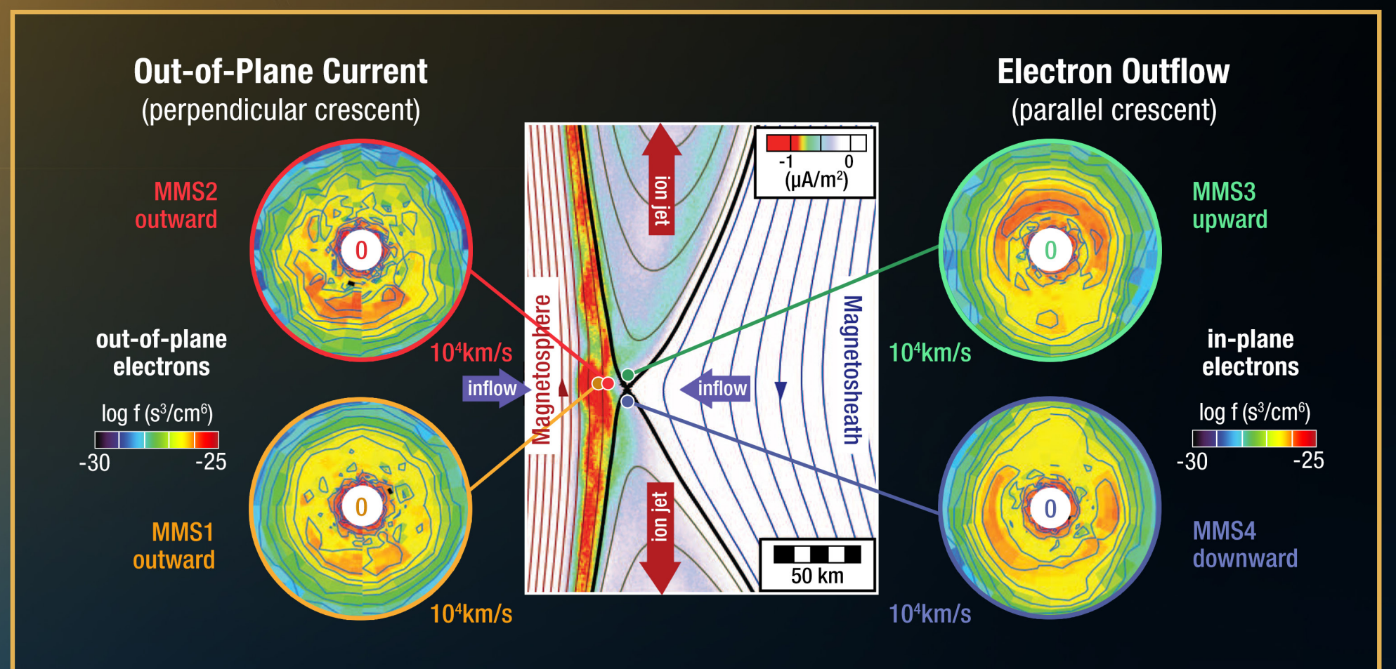
Electron dynamics controls the reconnection between the terrestrial and solar magnetic fields.
