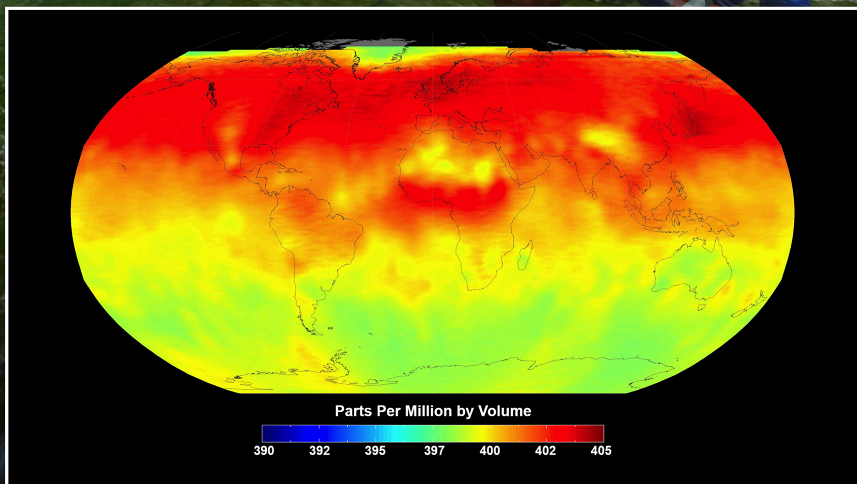
Atmospheric Carbon Dioxide Concentration – January 8 to 23, 2016
