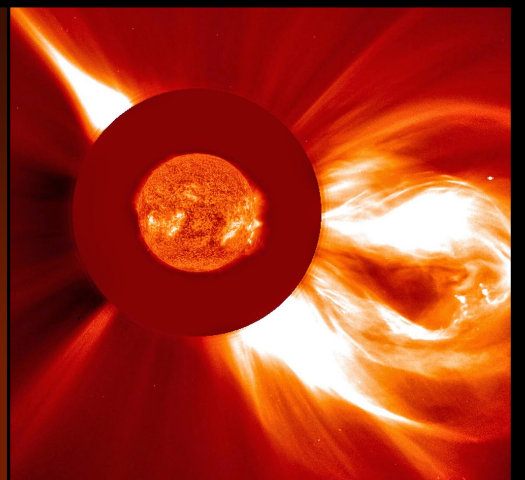
Parker will study the corona, the Sun's turbulent outer atmosphere.
