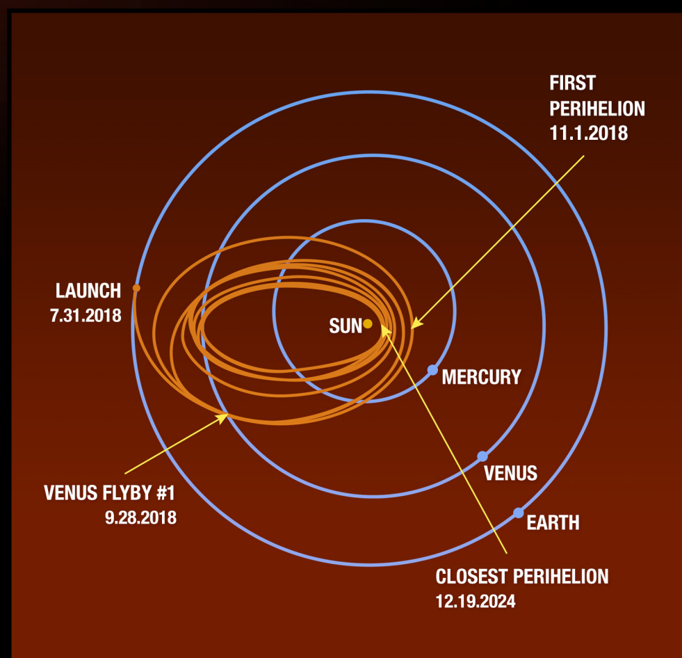
Using seven Venus gravity assists over seven years, Parker will pass within 10 solar radii of the sun.
