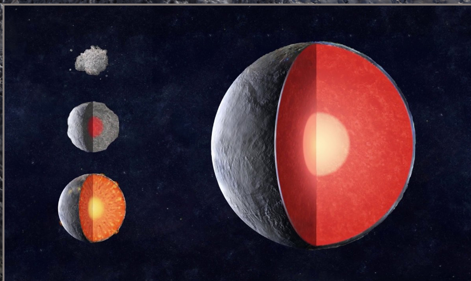
Located between Jupiter and Mars, 16 Psyche may be the core of an early planetesimal. This asteroid, likely composed largely of iron and nickel, could help us better understand Earth's core.
