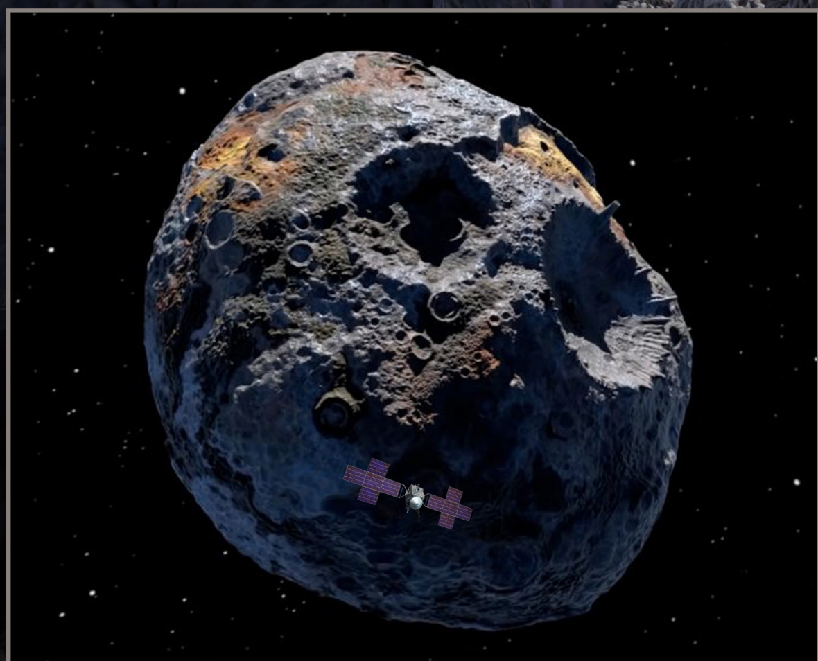
Asteroid 16 Psyche is approximately the size of Massachusetts.
