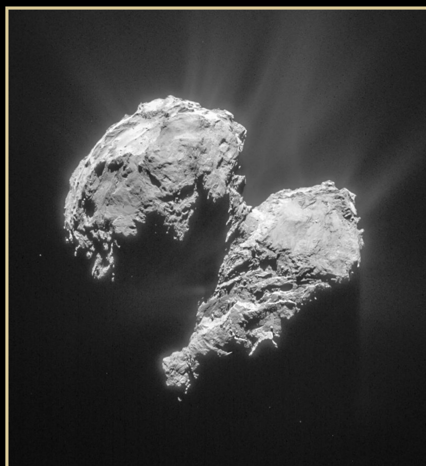
Rosetta approaches Comet 67P/Churyumov-Gerasimenko – March 22, 2015
