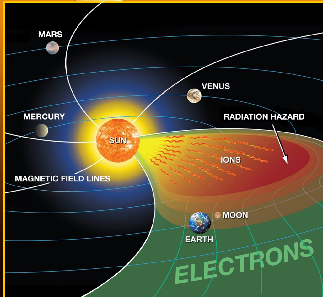
Sketch of solar particle event arrival at SOHO
