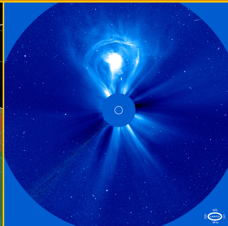
Coronal mass ejection – February 27, 2000
