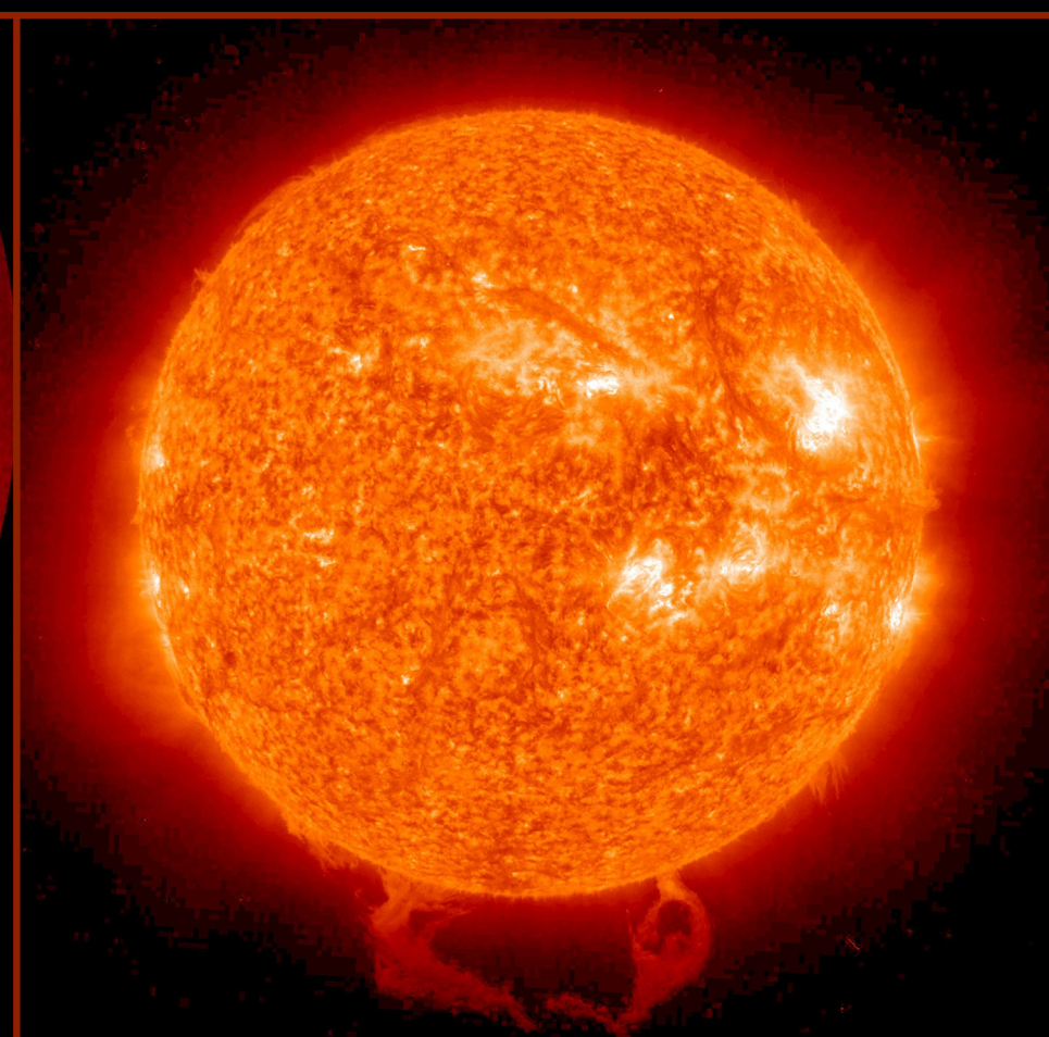
Double Prominence Eruptions – September 9, 2013
