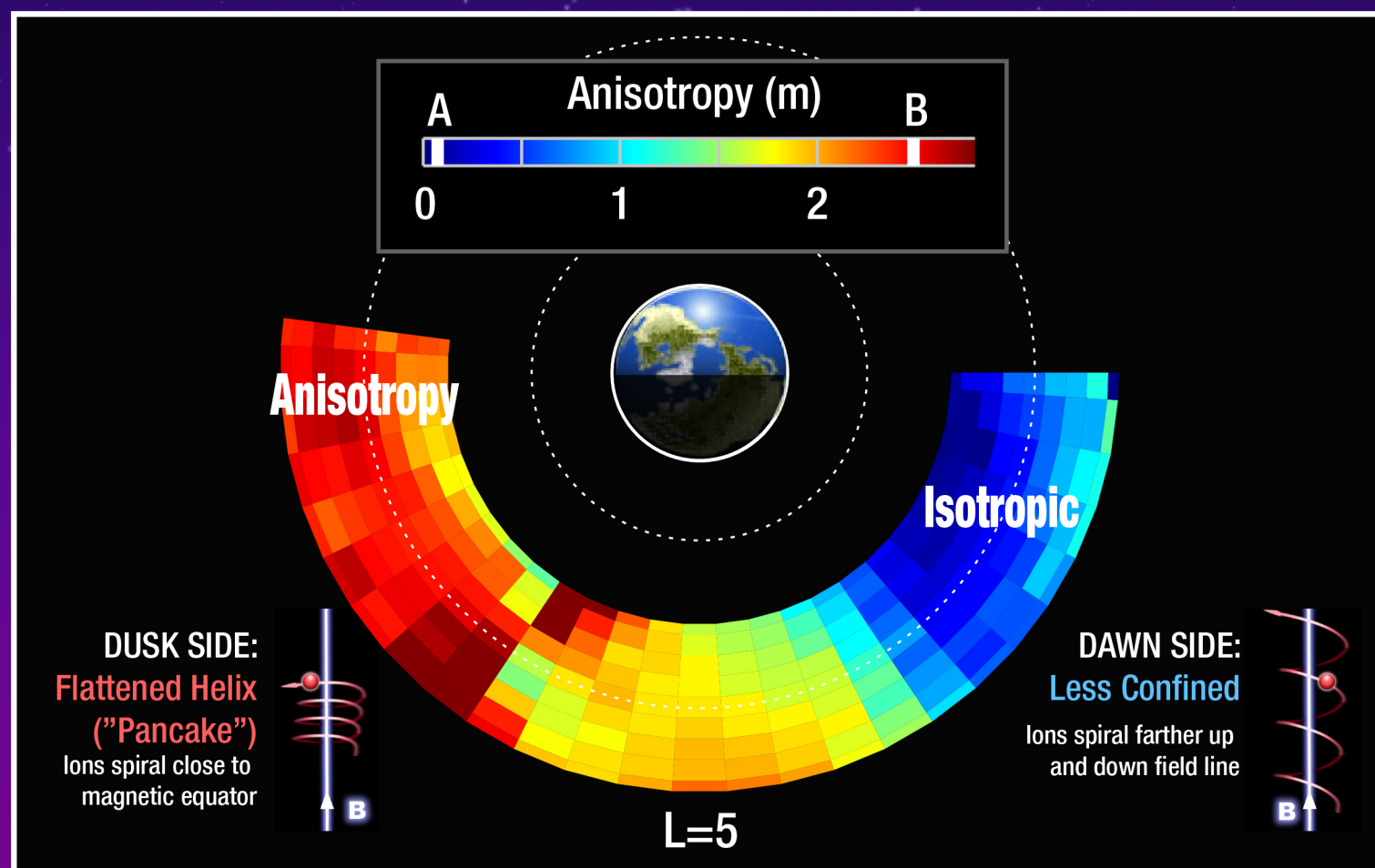
Obtaining images from two vantage points lets TWINS observe three dimensional structure, to determine ion anisotropy, or how close to the magnetic equator ions are trapped – April 6, 2010
