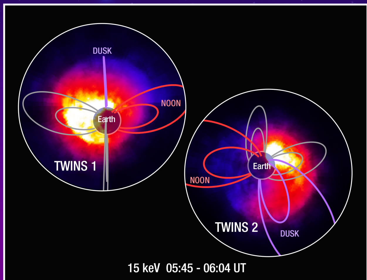
Stereo images from the first CME-driven storm of solar cycle 24 – April 6, 2010
