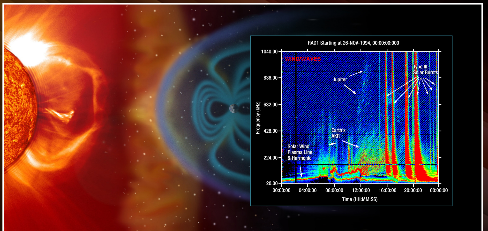
Heliophysics radio and plasma wave phenomena identified in Wind observations – November 26, 1994
