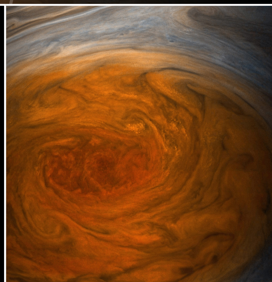
Jupiter's Great Red Spot – July 7, 2017
