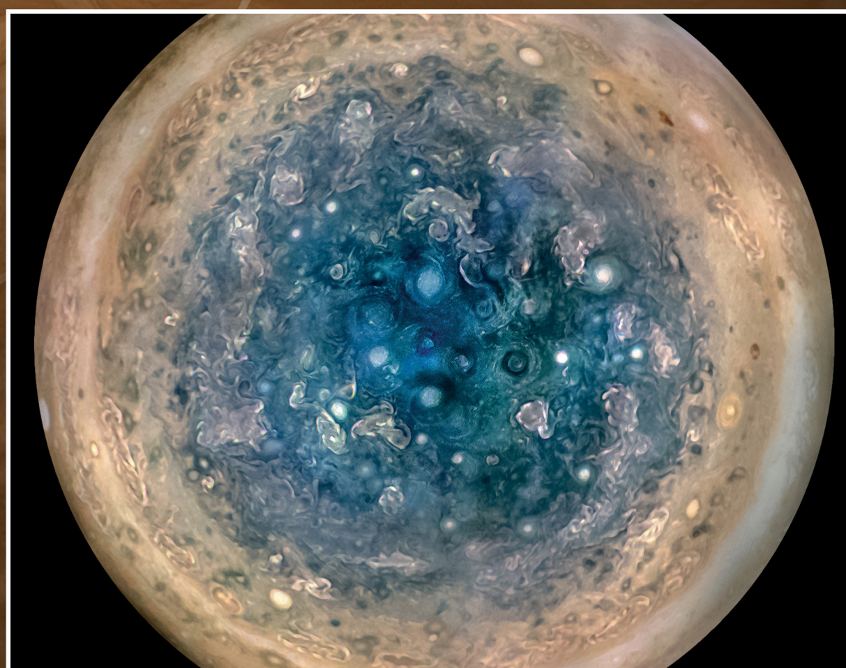
Jupiter's South Pole – May 25, 2017
