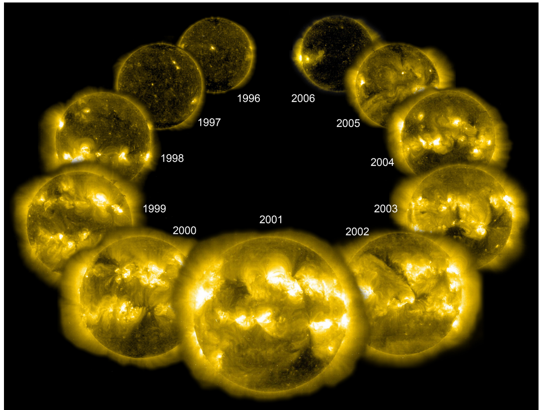
During periods of peak activity (front three images) sunspots, solar flares and coronal mass ejections are more common, and the sun emits slightly more energy than during periods of low activity (back images).
