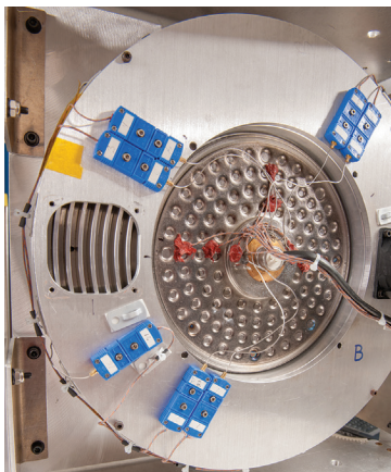
The Radial Core Heat Spreader shown mounted inside the experiment heat exchanger during preparations for the suborbital flight test.
