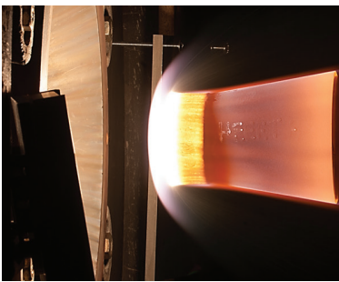
Testing of HEEET material at the NASA Ames Arc Jet Complex in the Interaction Heating Facility.
