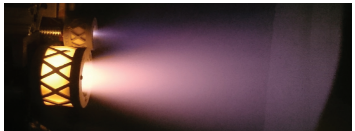
Busek's 65W iodine-fueled ion propulsion system "BIT-3," currently scheduled to fly on the LunaH-Map and Lunar IceCube missions.
