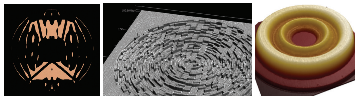
Pupil-plane reflective mask for the SPC, 24-mm diameter, black silicon on mirror (left). Image-plane reflective mask for the back-up technology Phase Induced Amplitude Apodization Complex Mask Coronagraph (PIAA-CMC) coronagraph, 155- \mu m diameter, raised elements on silicon (center). Image-plane transmitting mask for HLC, 100- \mu m diameter, raised dielectric and metal on glass (right). All masks were fabricated in the Micro-Devices Lab (MDL) at the Jet Propulsion Laboratory (JPL).
