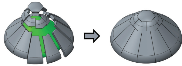
A drawing of the individual components that make up a heat shield (left) and the fully assembled heat shield with integrated seams bonded to the structure underneath (right).
