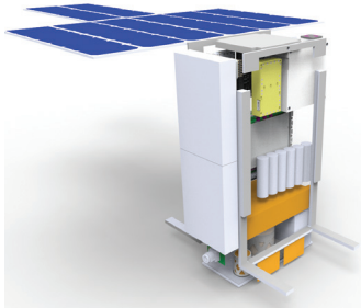
LunaH-Map Spacecraft Design (cutaway views).
