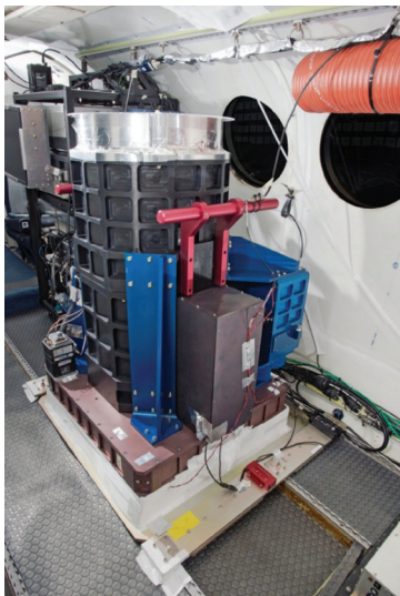
The 2 micron IPDA lidar system installed in the NASA B200. (Image credit: Upendra Singh)
