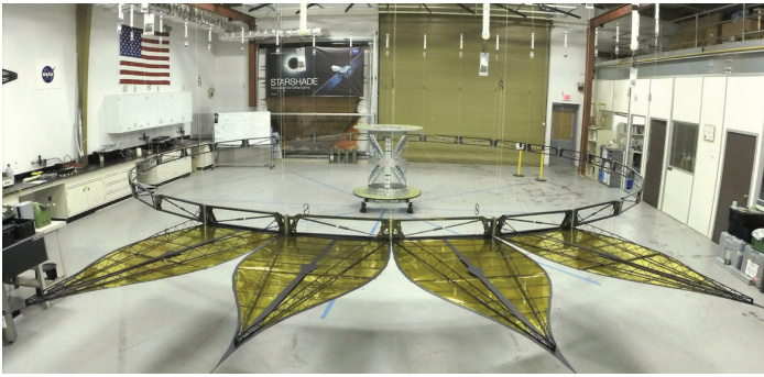
A 10-m prototype of the starshade's inner disk is demonstrated at NASA's Jet Propulsion Laboratory.
