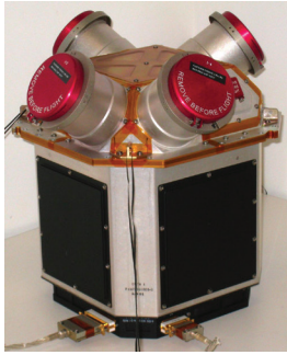
This cluster of four colloid thrusters is part of the Disturbance Reduction System, developed by NASA/JPL, which will help keep the LISA Pathfinder spacecraft extremely stable. (Image credit: ESA/NASA/JPL-Caltech)
