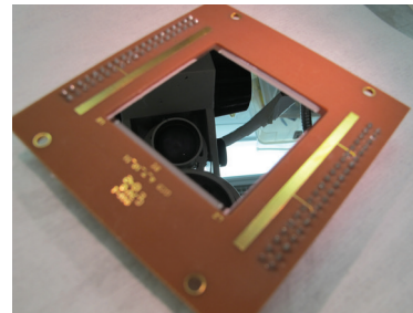
2-D-doped p-channel CCD for future Orion mission, CHESS rocket, and Mount Bigelow observation runs. (Credit: Todd Jones)
