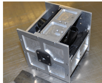
Left: Electric field booms compactly stowed in the CubeSat volume (10 cm on a side). Right: Six booms extend sensors from the main CubeSat body to distances of 5m, tip-to-tip, enabling tri-axial or vector electric field measurements. (Credits: CTD and NASA GSFC)
