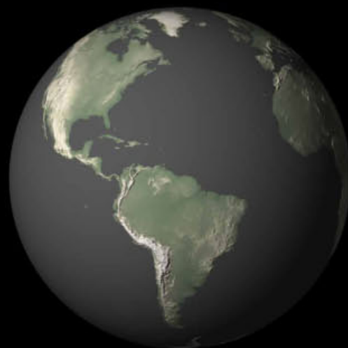
ASTER Elevation
