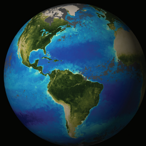
MODIS Biosphere
