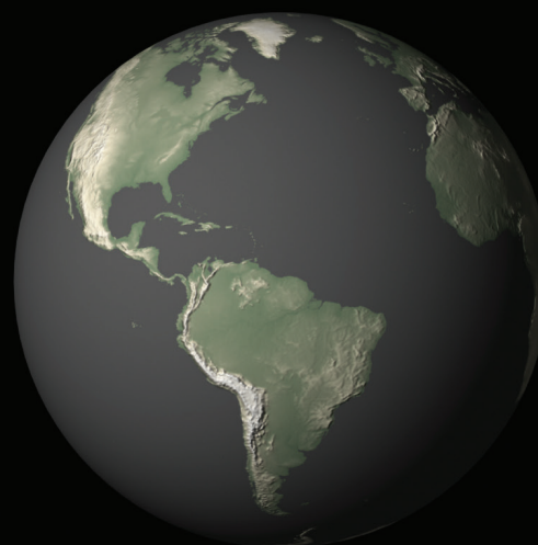
ASTER Elevation
