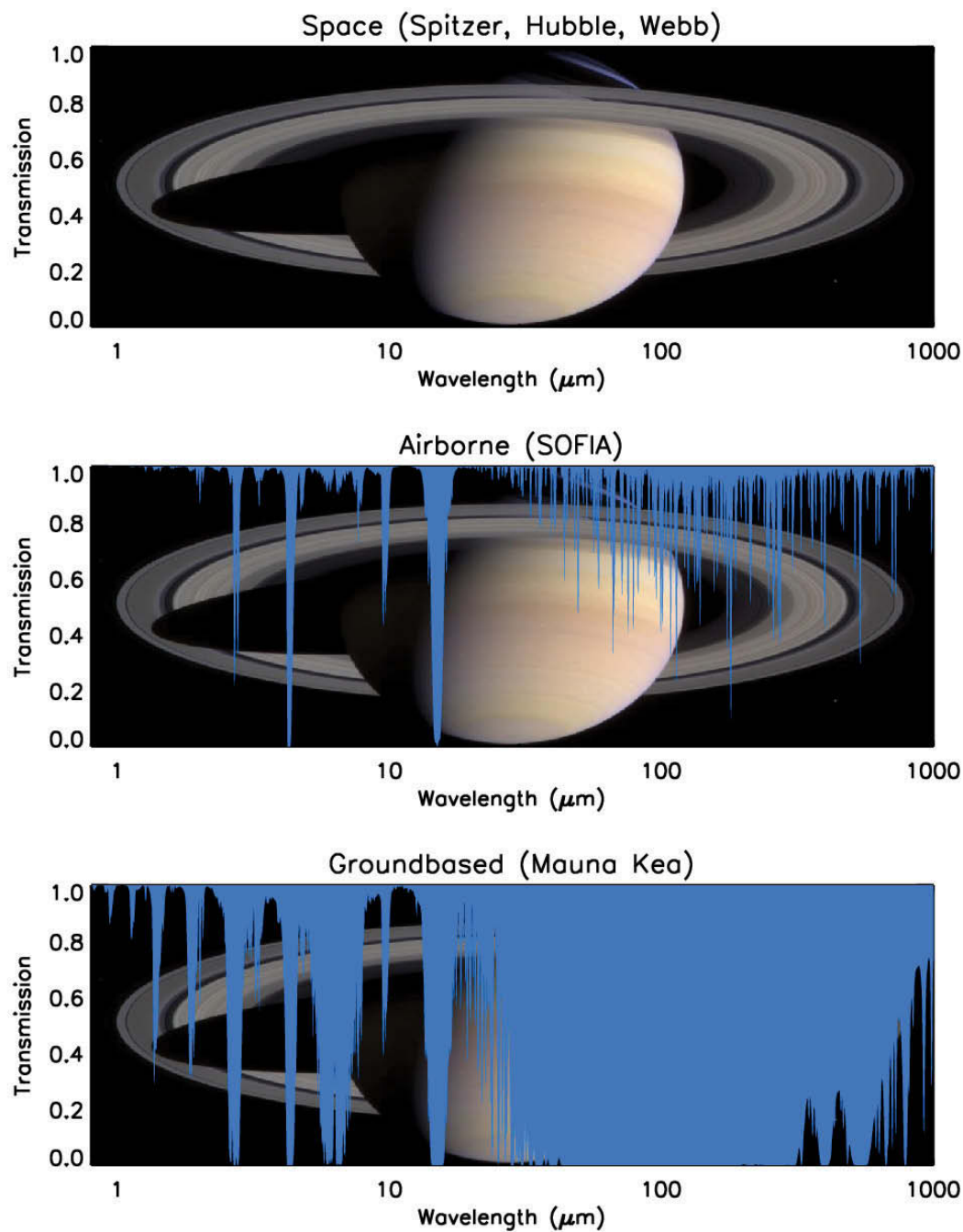
FIGURE 7.10 Earth's atmosphere blocks light from space, driving the need for telescopes at high altitudes. Bottom: On Mauna Kea ( \sim 14,000 feet above sea level), Earth's atmosphere transmission is reduced to zero throughout much of the infrared regime; many windows in the near infrared are blocked as well. Middle: The airborne Stratospheric Observatory for Infrared Astronomy (SOFIA) reduces these losses by operating above the bulk of the atmosphere; at about 45,000 feet, the measured average transmission from 1 to 1,000 \mu\text{m} is equal to or greater than 80 percent except in the center of absorption lines due to mostly telluric \text{H}_2\text{O} , \text{CO}_2 , and \text{O}_2 . Top: Spaceborne telescopes such as Hubble, Herschel, Spitzer, and Webb are completely free of such effects. SOURCE: Spectra from www.spectrafactory.net , courtesy of Andrew Markwick and Jan Cami; Saturn image PIA06193, courtesy of NASA/JPL/Space Science Institute; composite created by Tim Warchocki.
