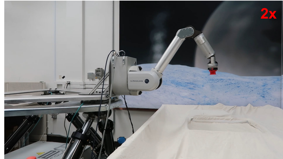
Earth Gravity
