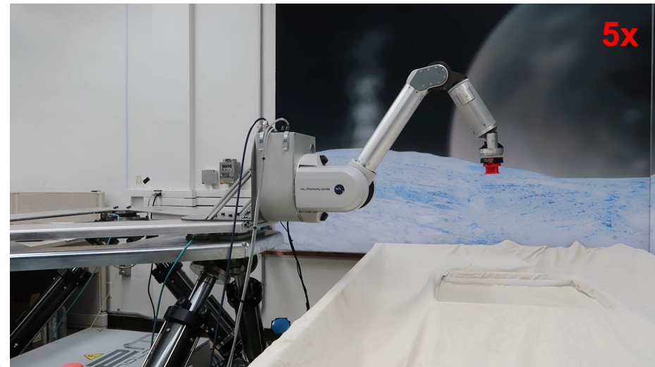
Enceladus Gravity
