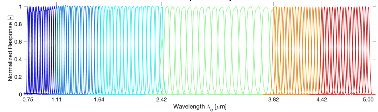
SPHEREx Spectral Response
