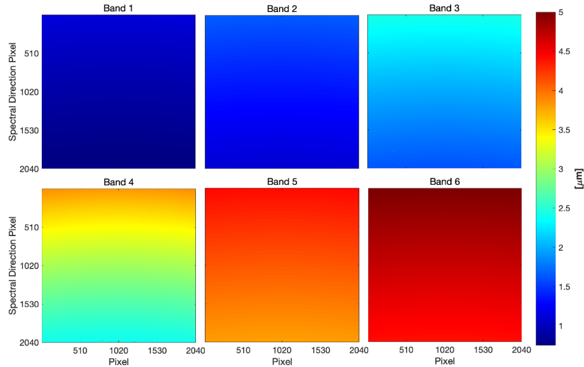
SPHEREx Band Center \lambda_c
