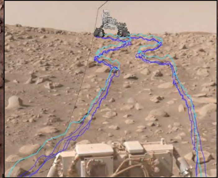
Annotated composite image shows the path Perseverance took through a dense section of boulders. The pale blue line indicates the course of the center of the rover's front wheel hubs, while the darker blue lines show the paths taken by the bottom of the rover's six wheels. Credit: NASA/JPL-Caltech
